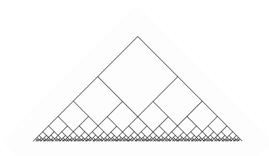
Figure 4: The hyperbolic graph S_{2,3} .
